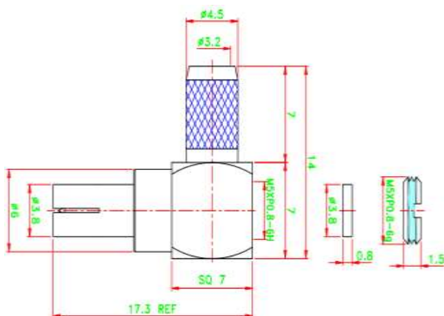
TS9 MALE R/A CONNECTOR FOR RG 58 AND 195 SERIES CABLE
