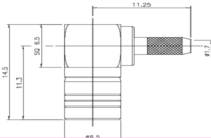
SMB FEMALE R/A RG 174, RG 316 CONNECTOR
