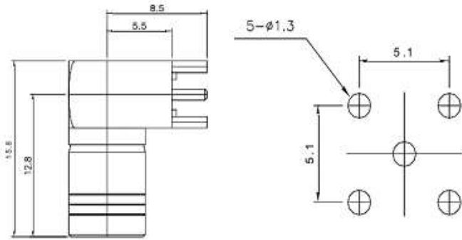
SMB FEMALE R/A PCB CONNECTOR
