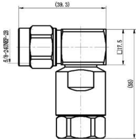
N Male R/A 1/2" Feeder Connector
