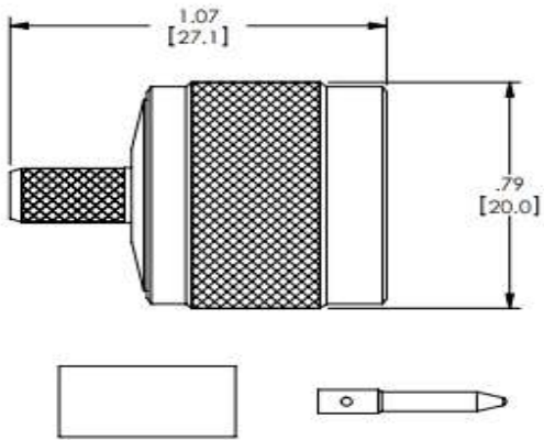
N Male LMR 200 Crimp
