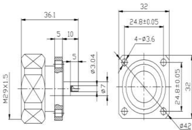
7/16 DIN Male 4 Hole Panel Mount
