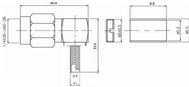
SMA Male RA for RG316 / 174 / LMR 100 Crimp Connector Part No. SRFS- SMAMRACRRG316 -06
