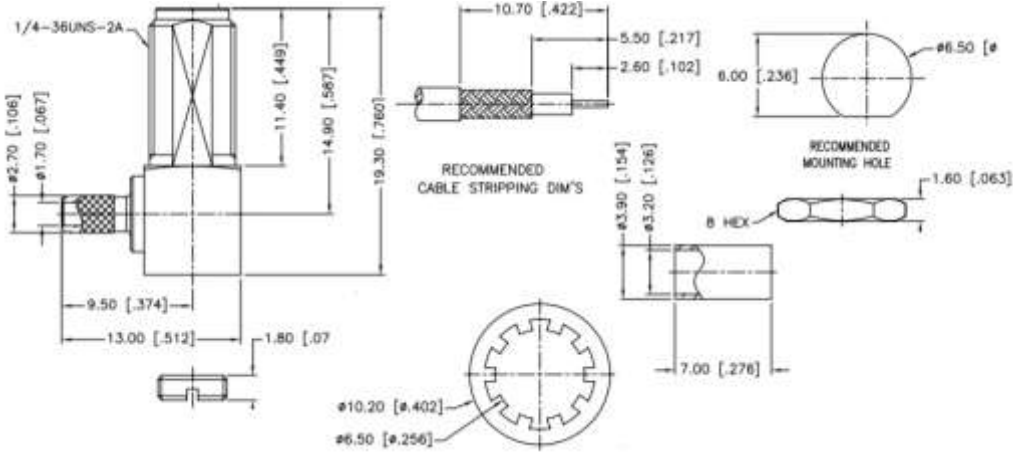
SMA Female RA for RG 316/Rg174 Crimp Connector Part No. SRFS- SMAFRACRRG316-06
