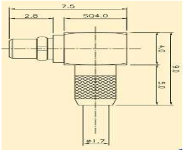
MMCX Male Right Angle RG178
