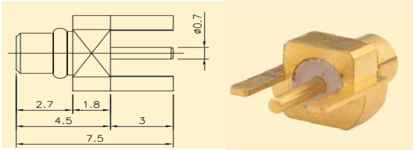
MMCX Male End Launch
