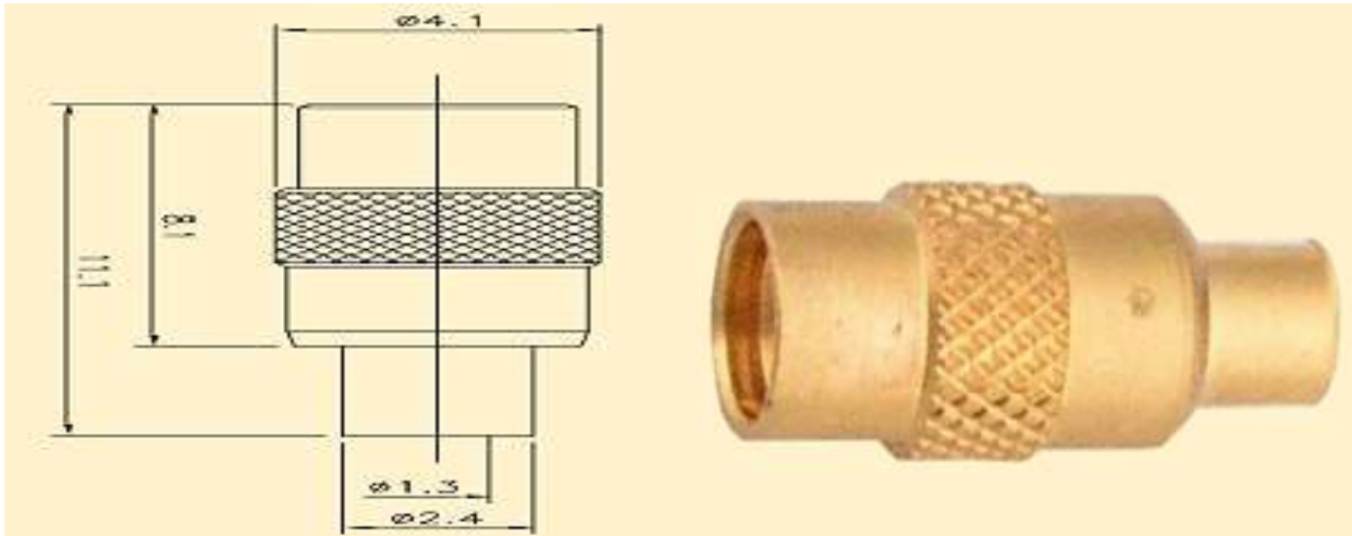
MMCX Female Straight SF047, SR047
