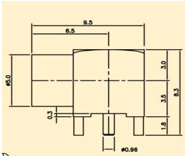
MCX Female RA PCB
