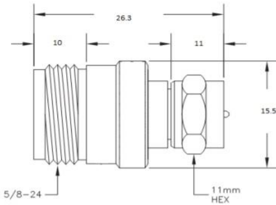
N Female to F Male Adaptor (SRFS-ANFFM04)
