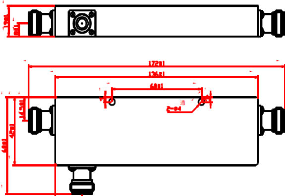
10 dB Directional Coupler
